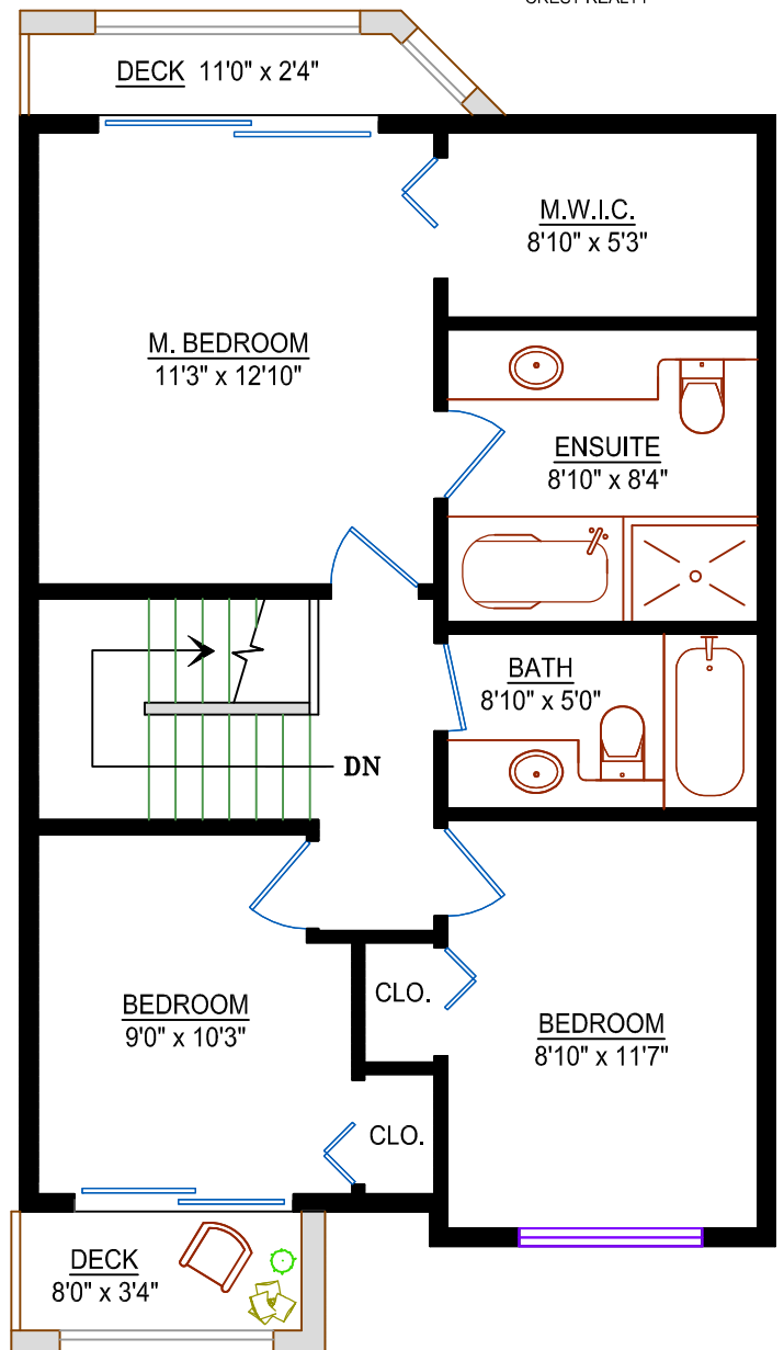
UPPER LEVEL Area: 663 sq. ft.
